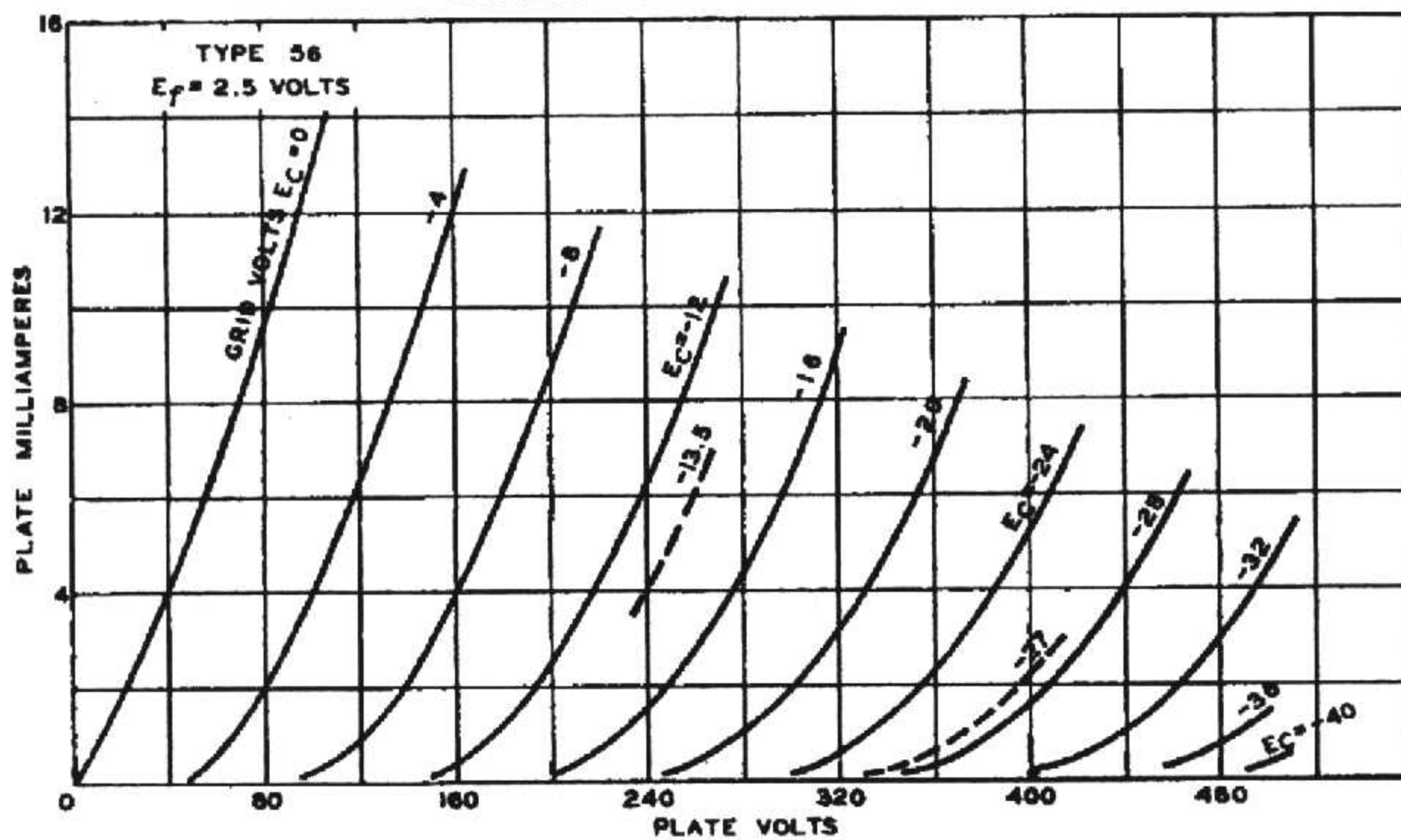
HIGH-GAIN AUDIO-FREQUENCY AMPLIFIER
