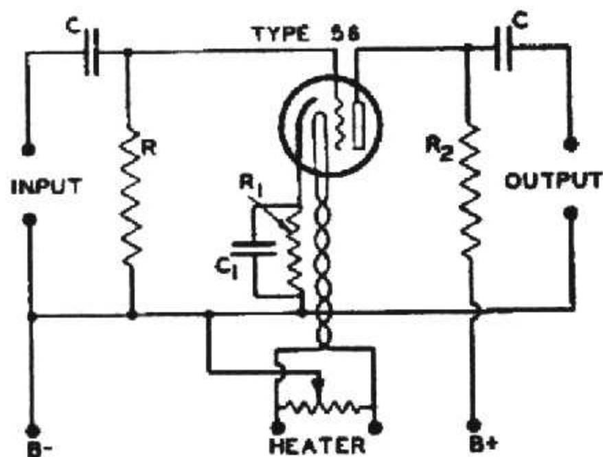
RESISTANCE-COUPLED A-F AMPLIFIER
