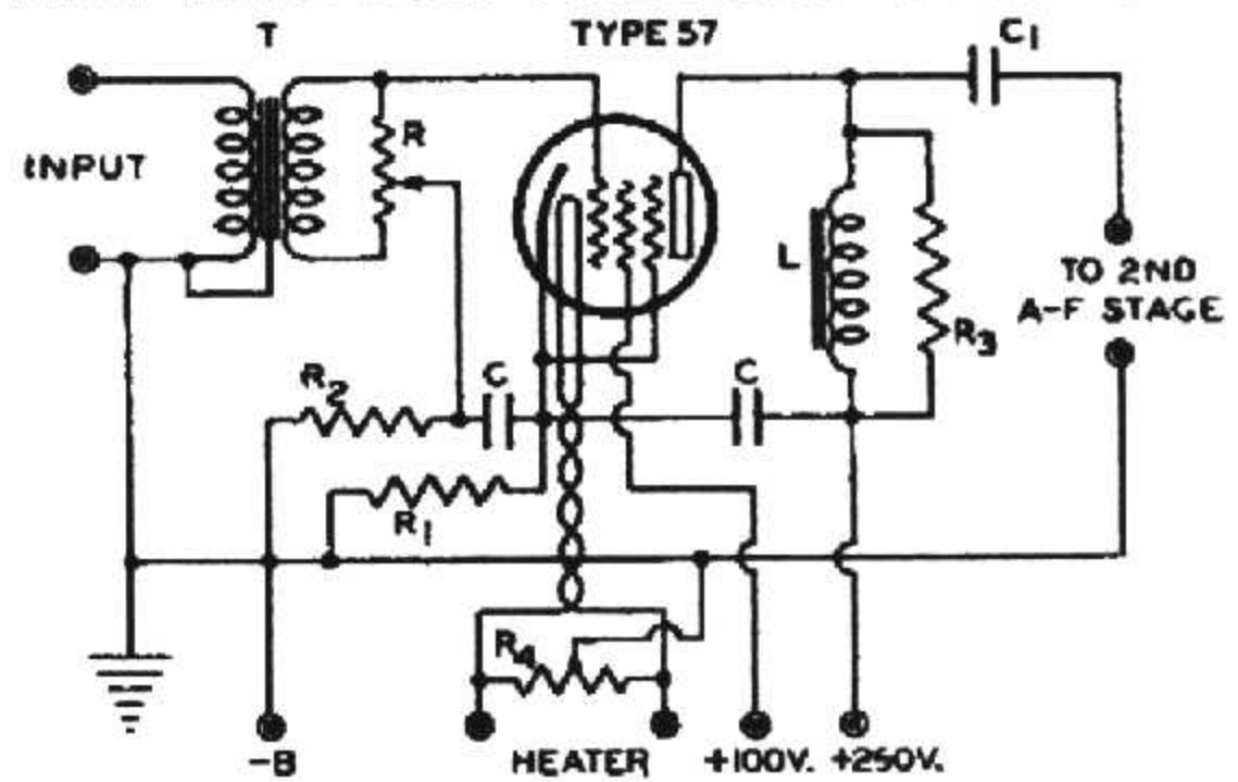
HIGH-GAIN AUDIO-FREQUENCY AMPLIFIER
